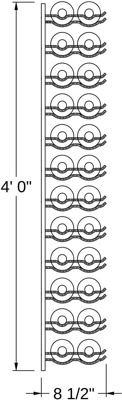
(Standard Mounting) Side View
