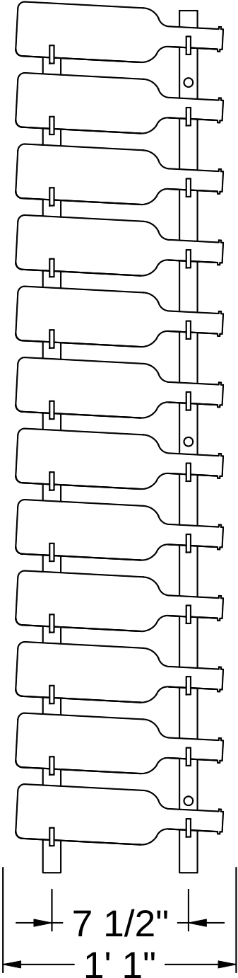
(Standard Mounting) Front View
