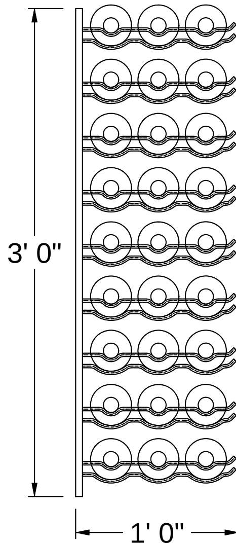
(Standard Mounting) Side View
