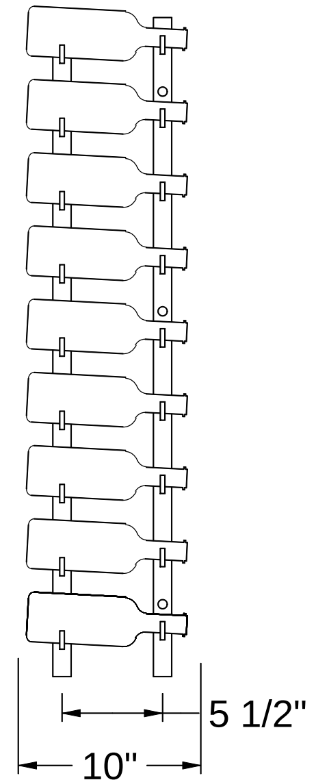
(Mounting for Splits) Front View
